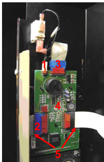
Photo 5 Affichage PCB
