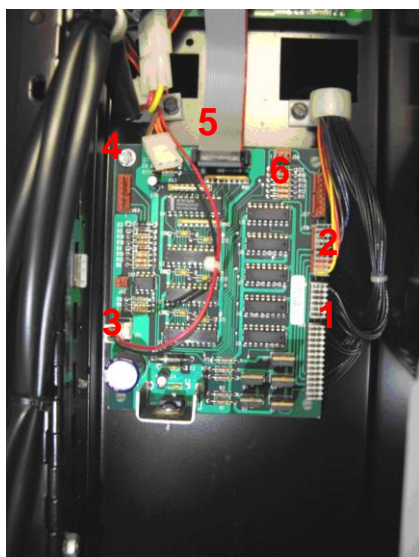
Photo 4 Interface PCB
