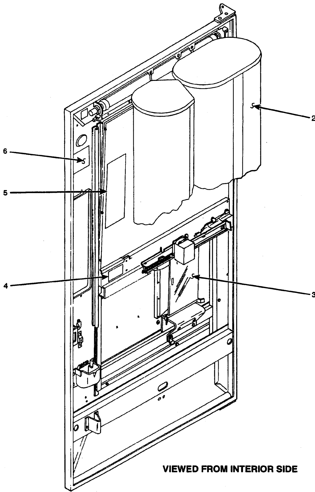
Figure 3. Door Assembly (Sheet 1 of 2)
