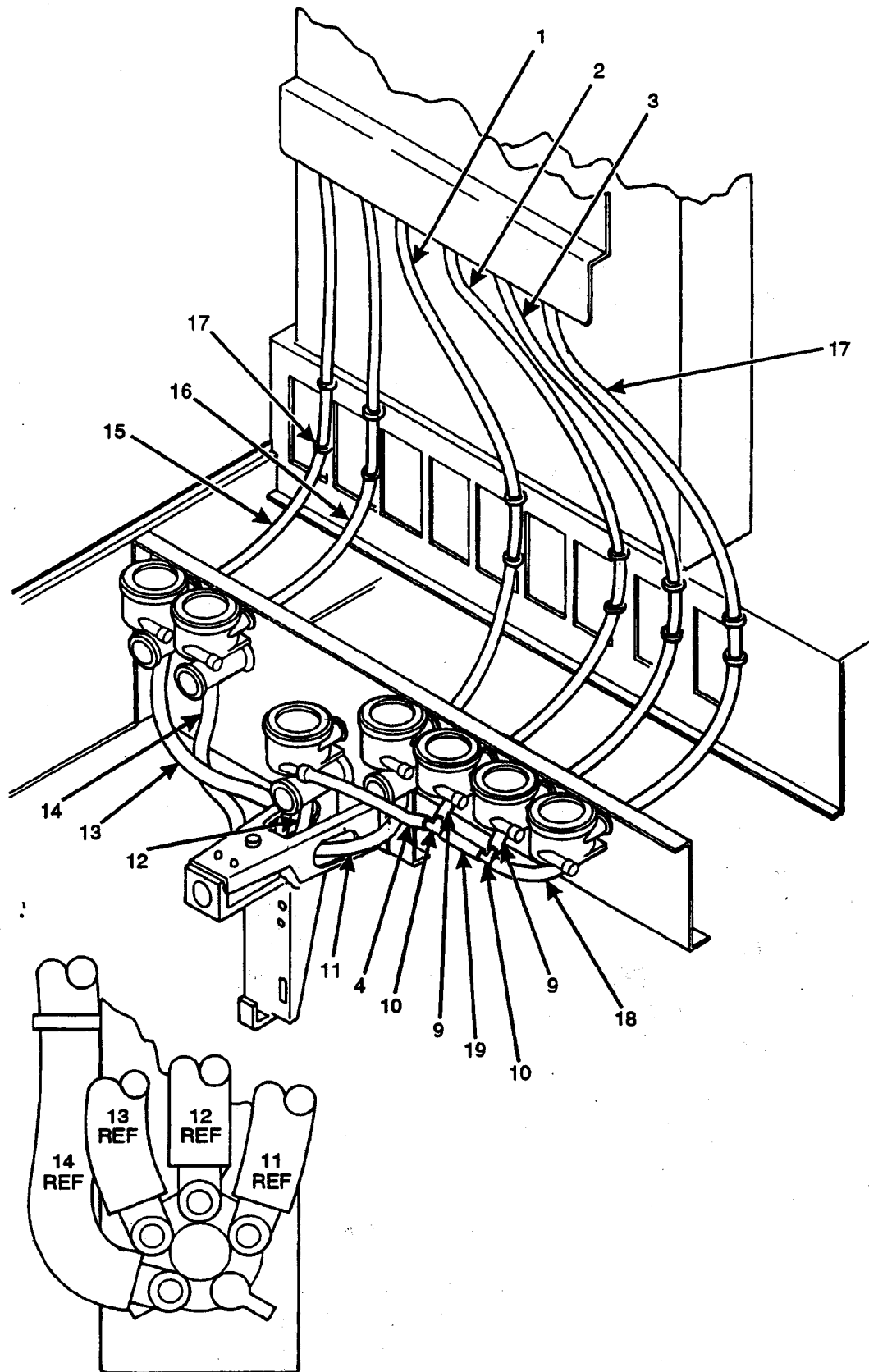
Figure 30-B. Liquid Distribution and Drain System, Part 2 (Sheet 3 of 3)
