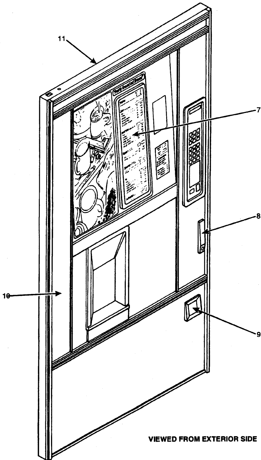
Figure 3. Door Assembly (Sheet 2 of 2)
