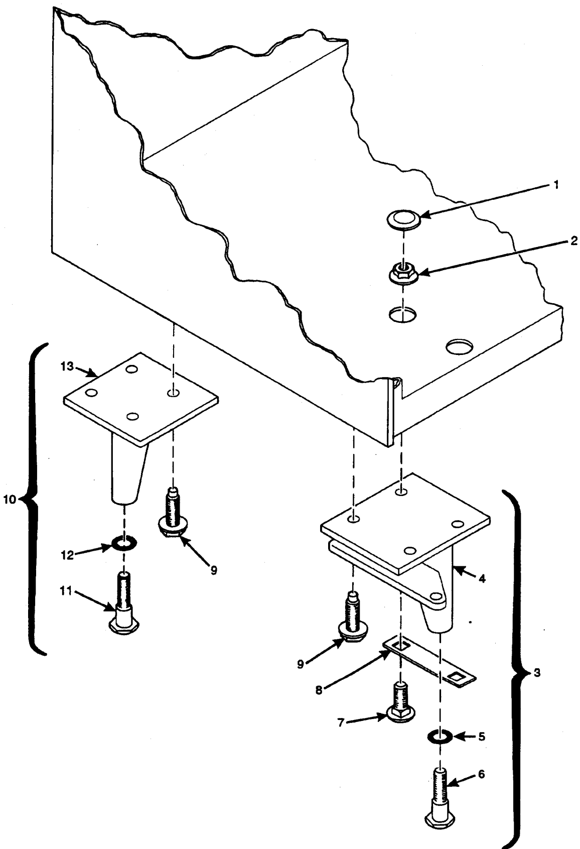
Figure 13. Leg, Leveler, and Leg and Hinge Assemblies
