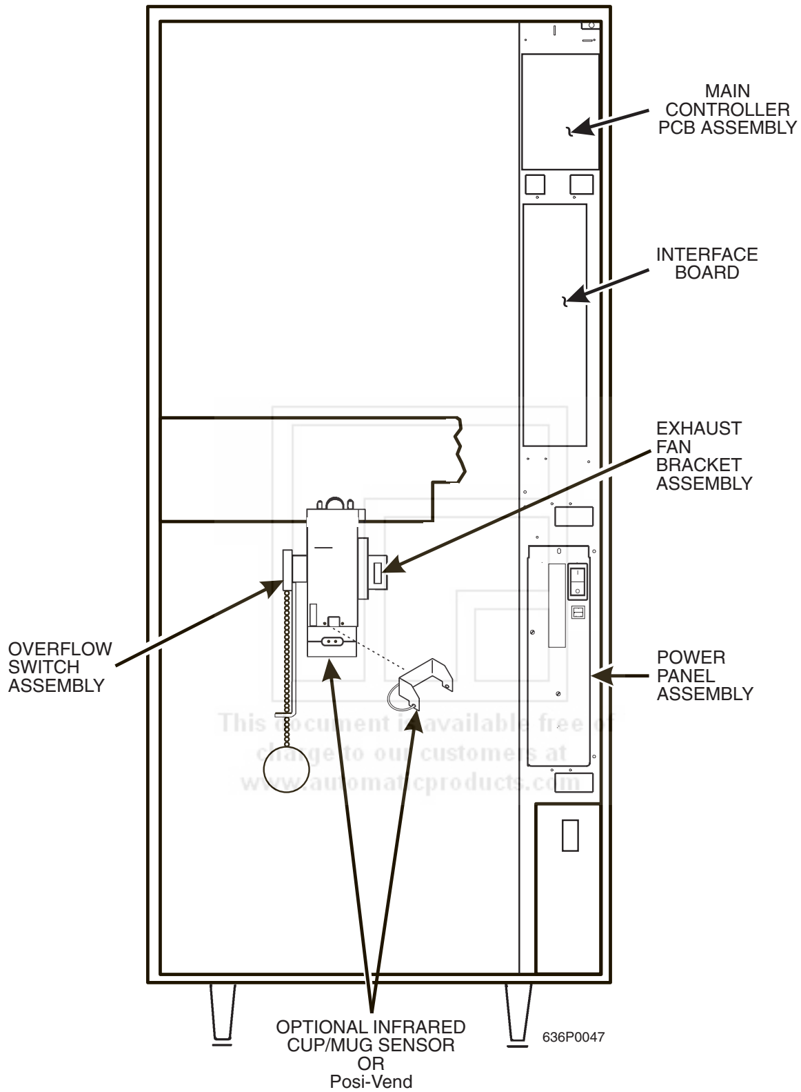
MERCHANDISER CABINET INTERIOR (FIGURE 2 OF 2)
